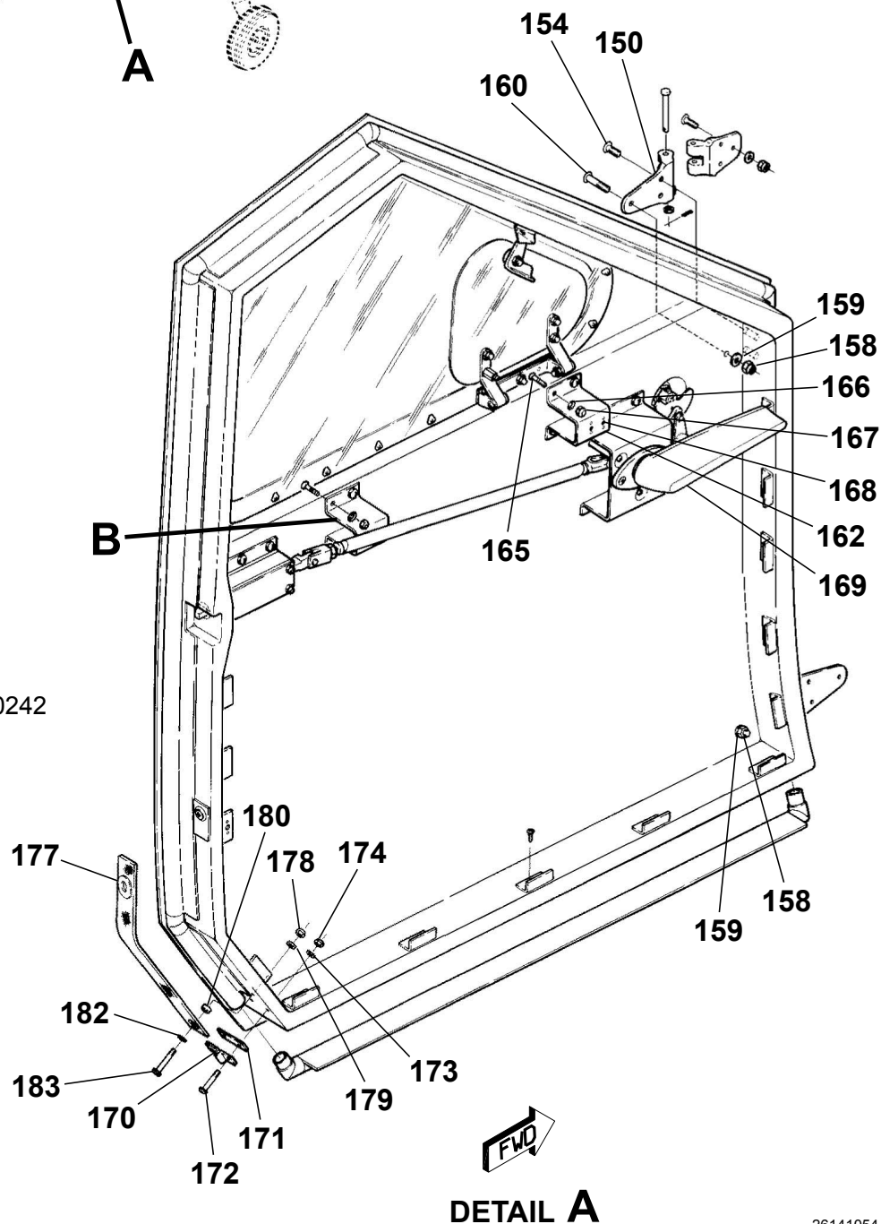
CREW DOOR ASSEMBLY Figure 01. (Sheet 3)
