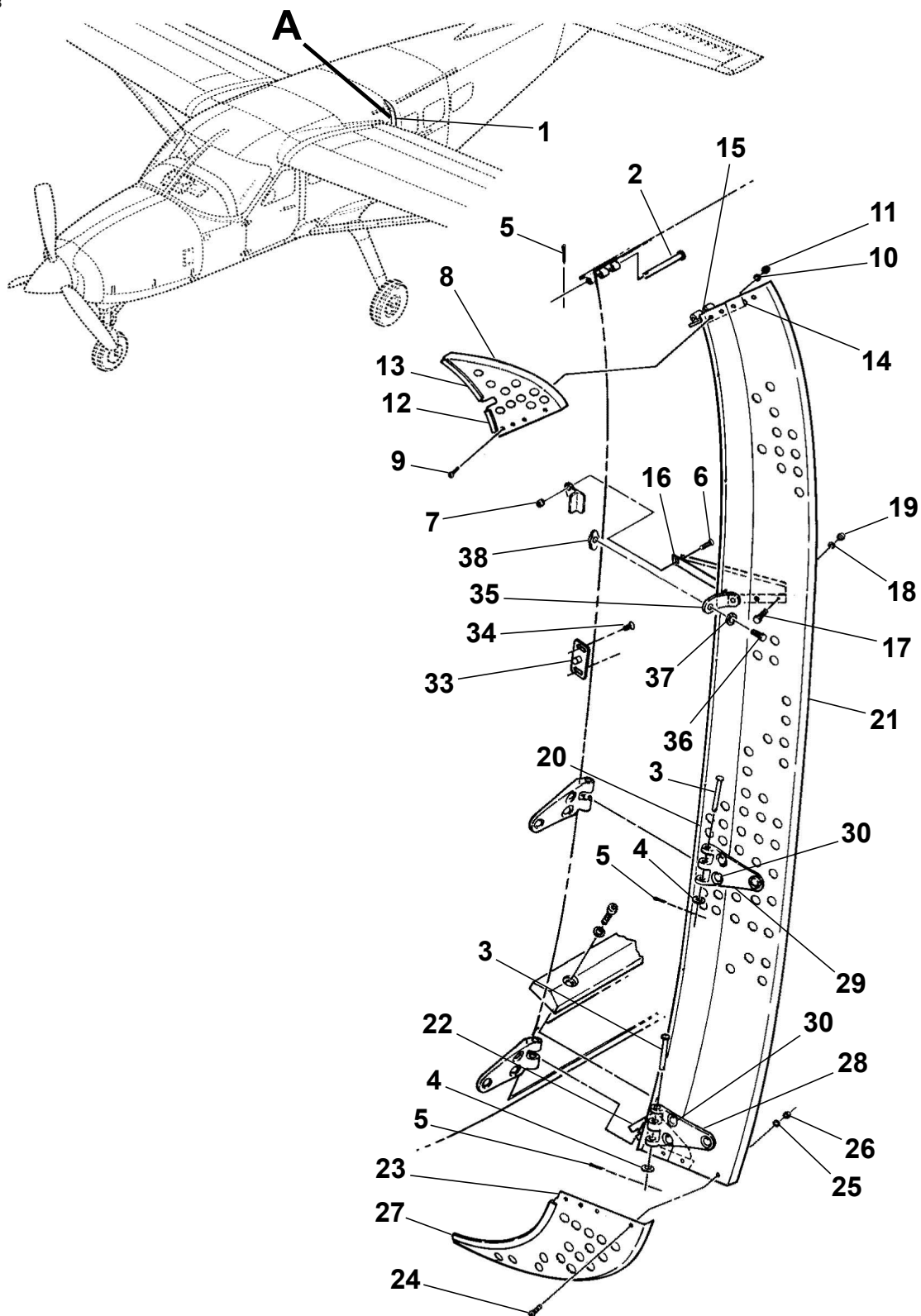
AIR DEFLECTOR INSTALLATION - CARGO DOOR Figure 01. (Sheet 1)
