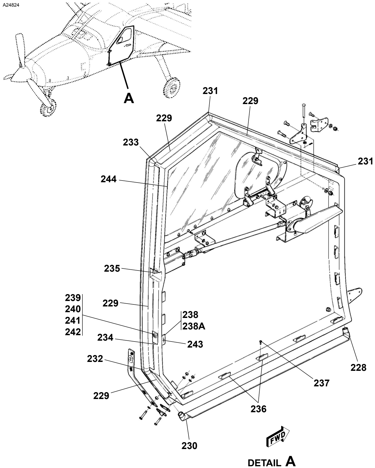
CREW DOOR ASSEMBLY Figure 01. (Sheet 4)
