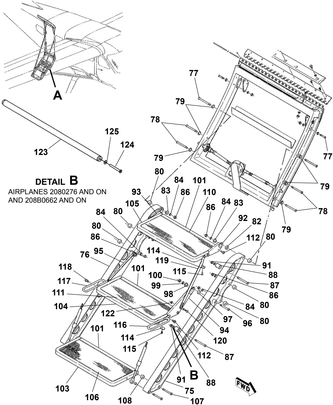
DETAIL A PASSENGER DOOR AND STEP INSTALLATION - LOWER Figure 01. (Sheet 2)
