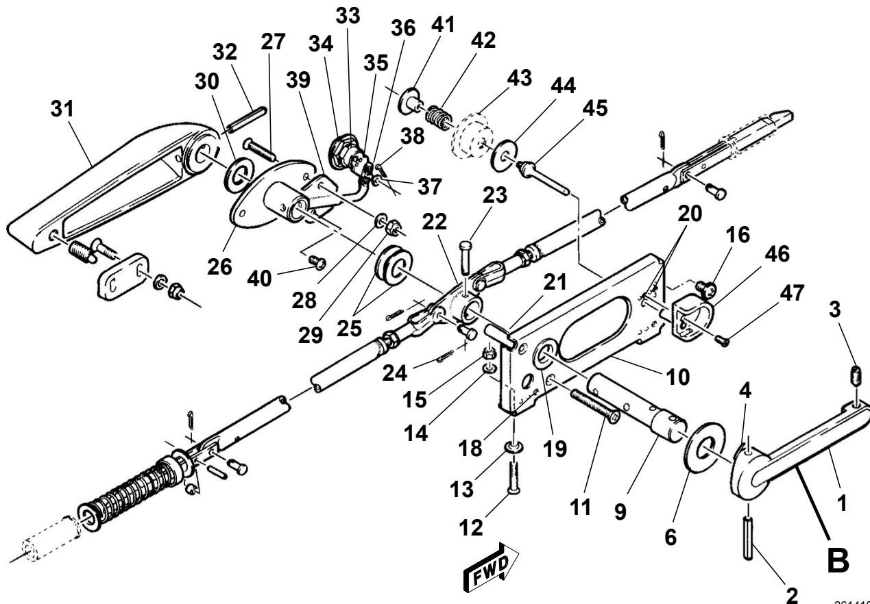
DETAIL A LATCH MECHANISM - UPPER CARGO DOOR Figure 03. (Sheet 1)
