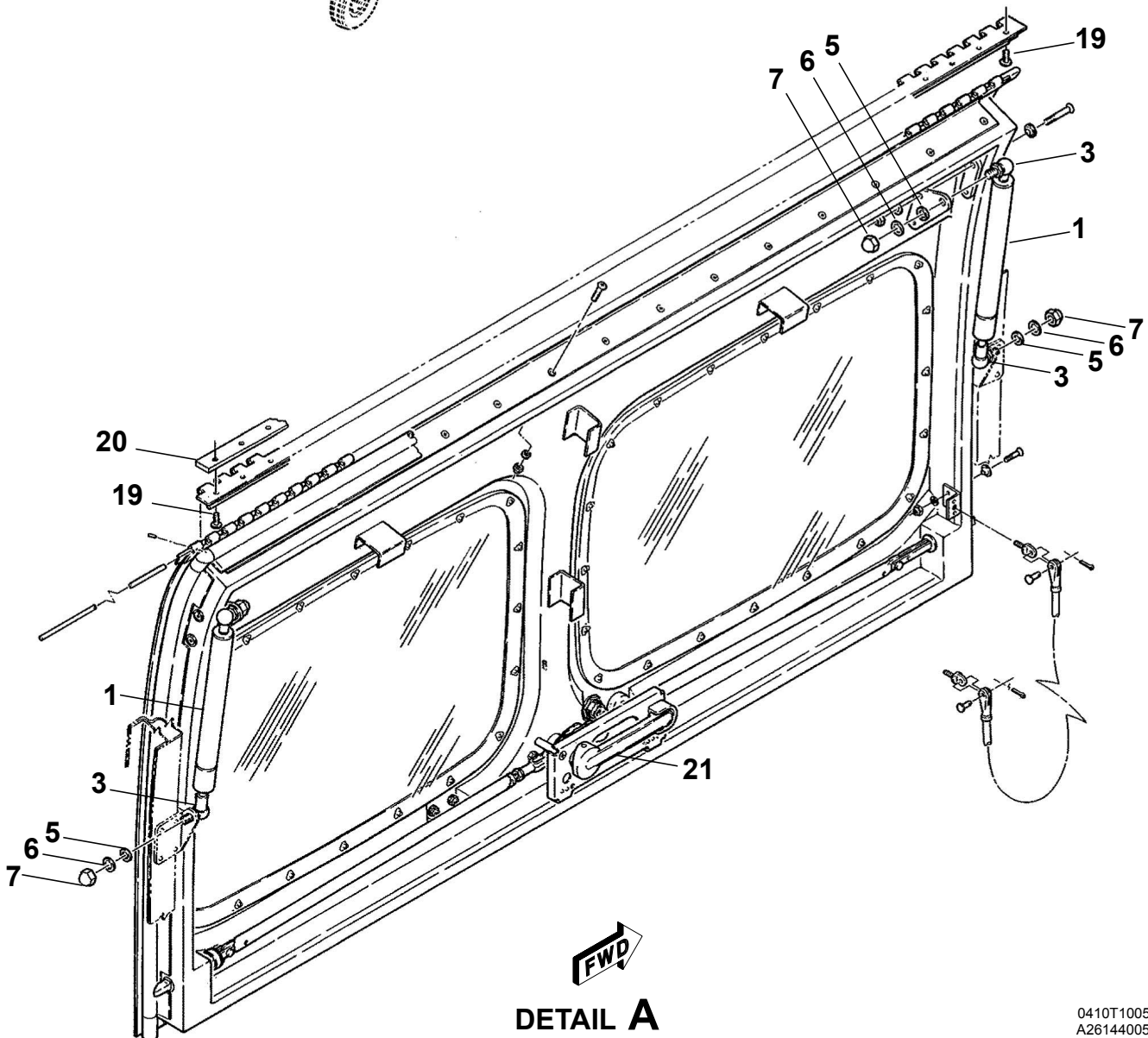
CARGO DOOR INSTALLATION - UPPER Figure 01. (Sheet 1)
