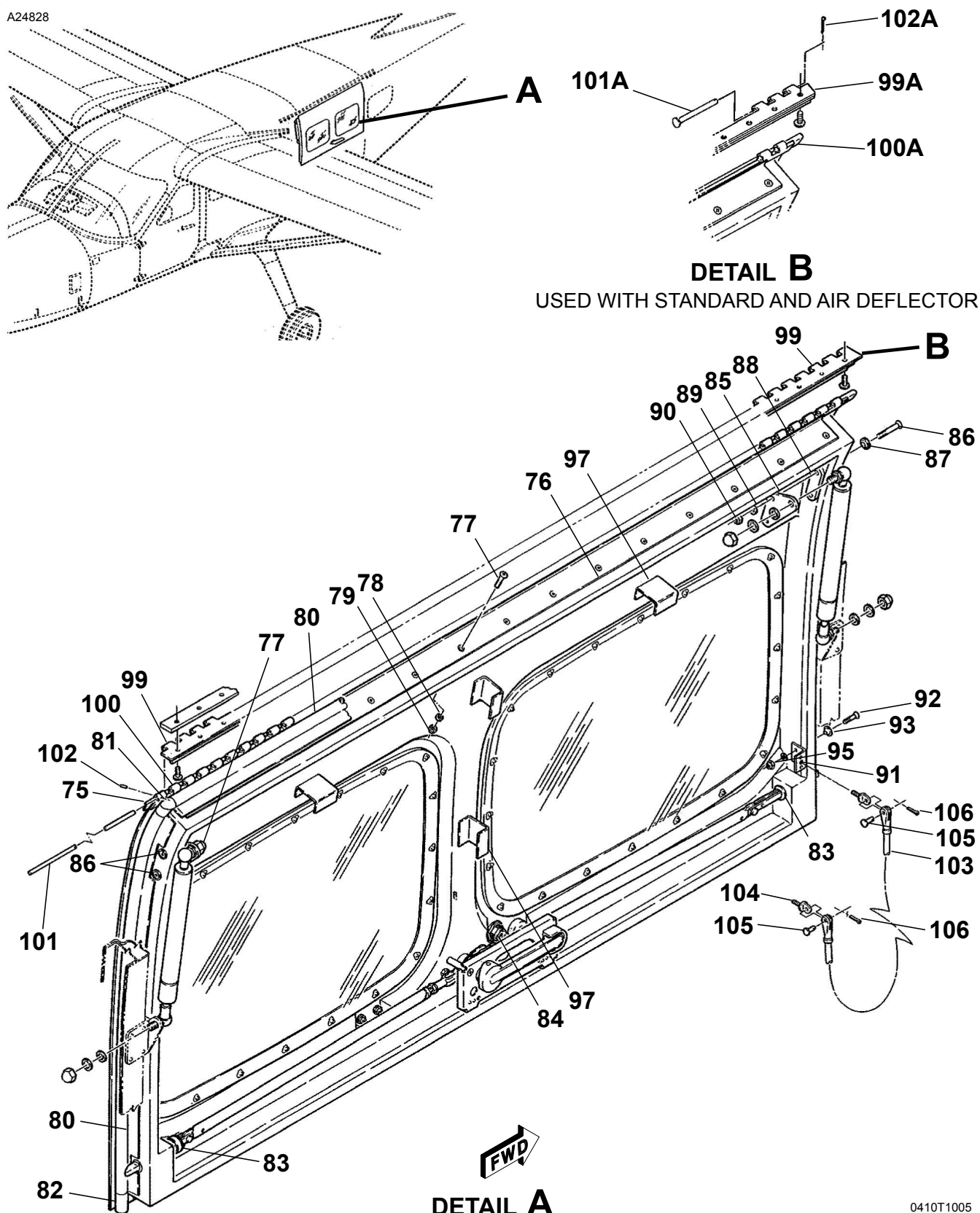
CARGO DOOR INSTALLATION - UPPER Figure 01. (Sheet 2)
