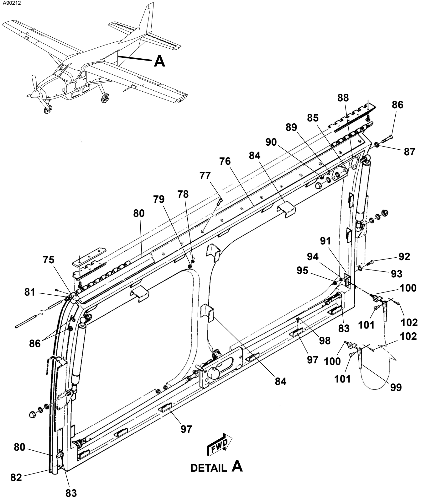
CARGO DOOR INSTALLATION - UPPER NOT USED ON PASSENGER VERSION Figure 02. (Sheet 2)
