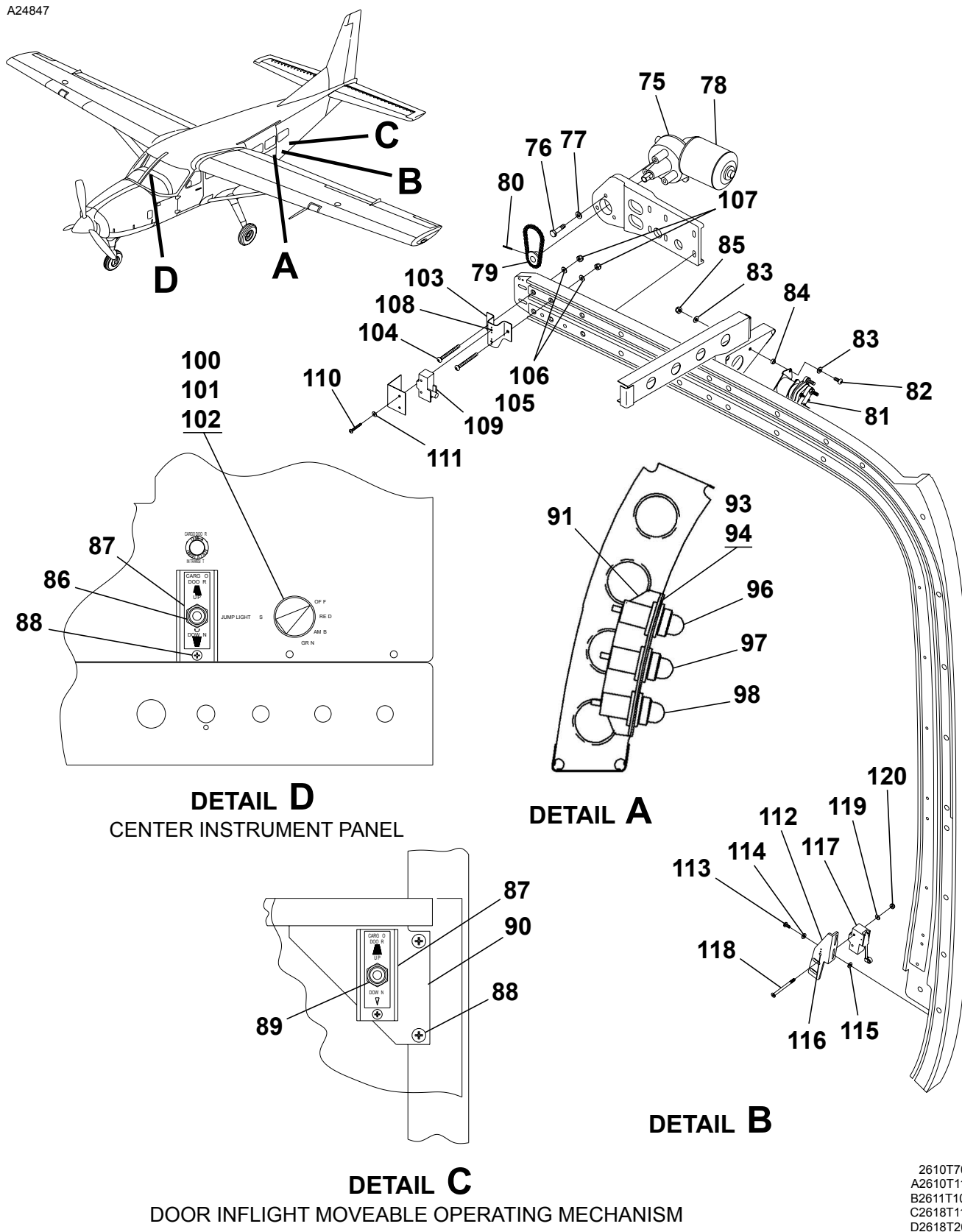
DOOR INFLIGHT MOVEABLE OPERATING MECHANISM Figure 02. (Sheet 2)
