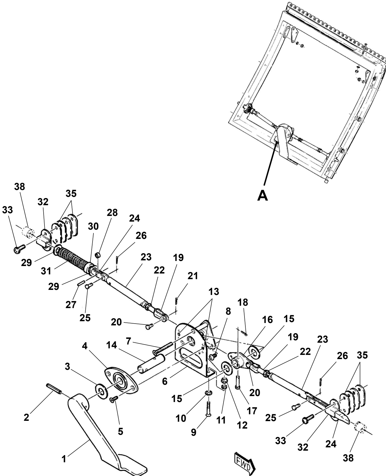
LATCH MECHANISM - LOWER PASSENGER DOOR Figure 02. (Sheet 1)
