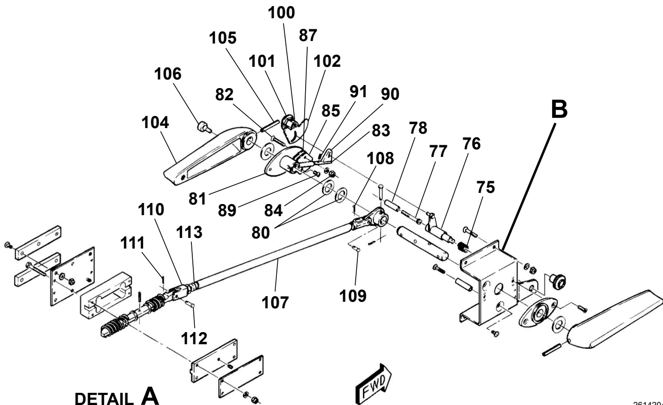
LATCH MECHANISM - CREW DOOR Figure 02. (Sheet 2)
