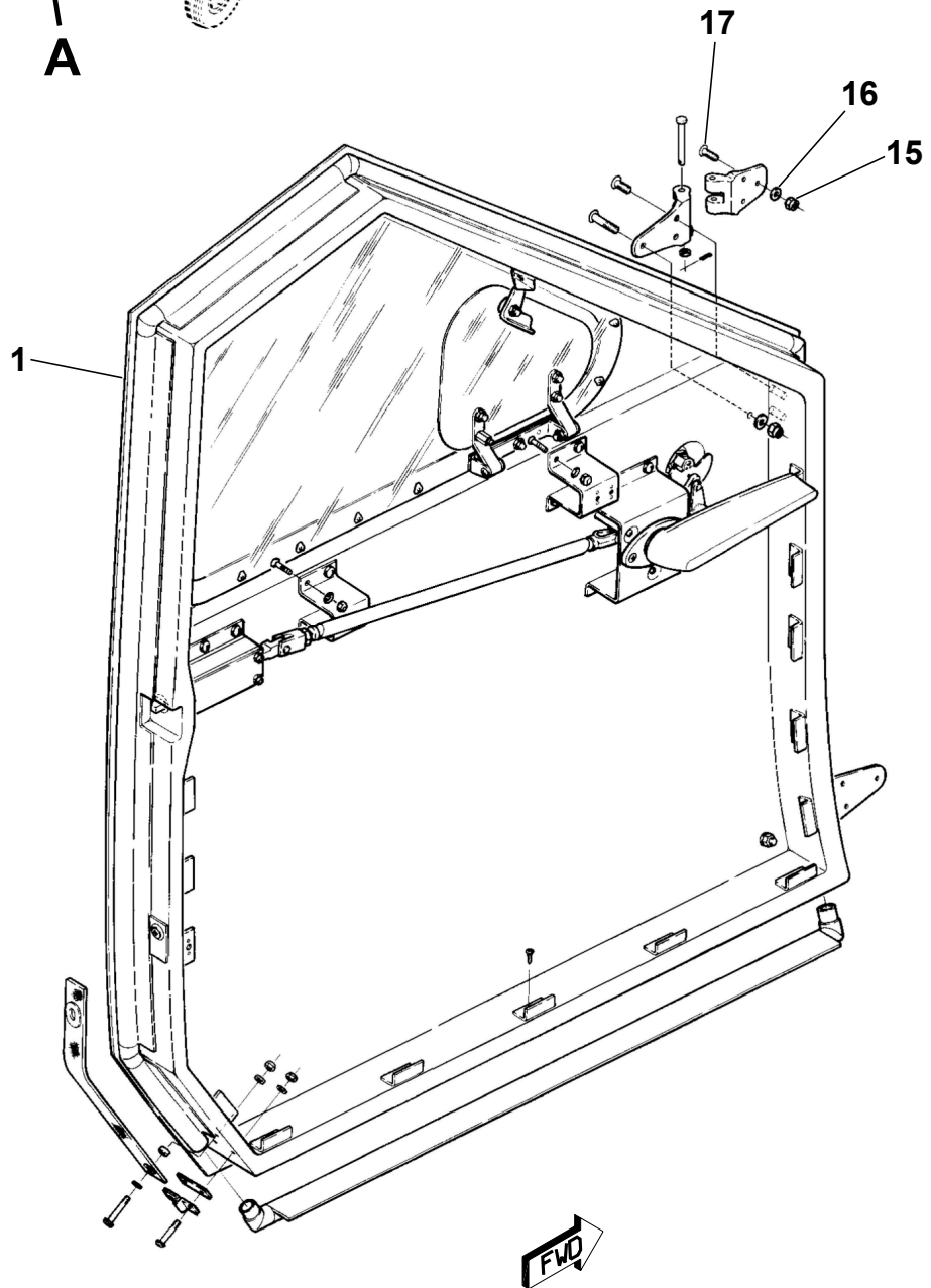
CREW DOOR ASSEMBLY Figure 01. (Sheet 1)
