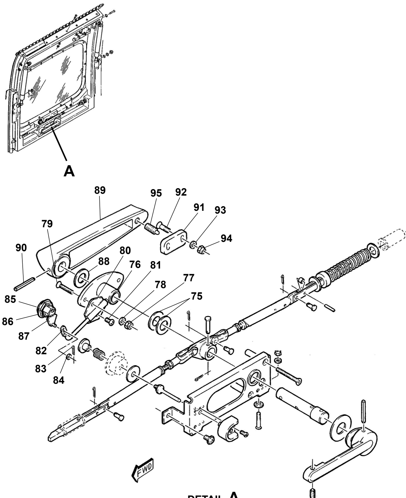
LATCH MECHANISM - UPPER PASSENGER DOOR Figure 02. (Sheet 2)
