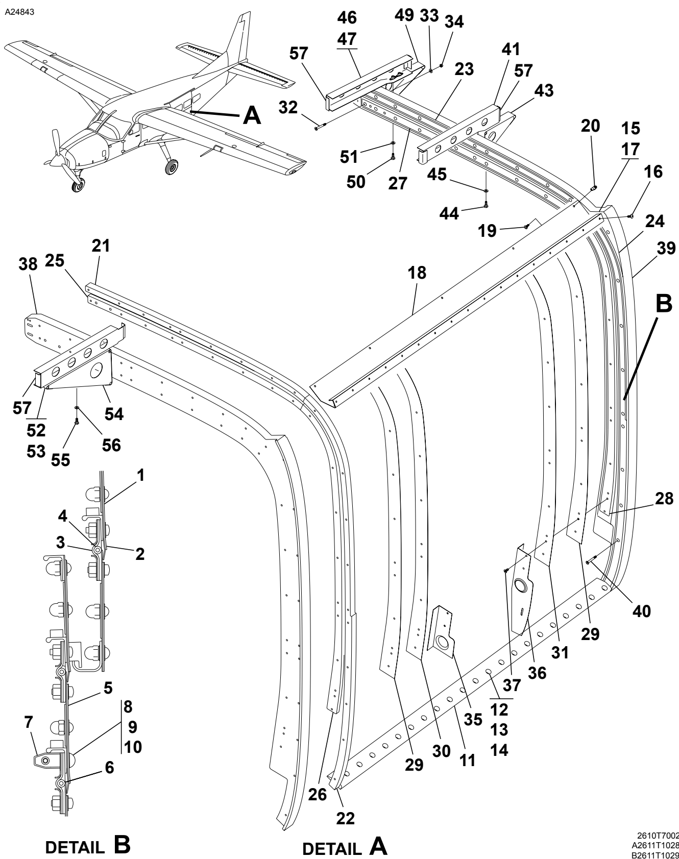
DOOR INSTALLATION - INFLIGHT MOVEABLE Figure 01. (Sheet 1)
